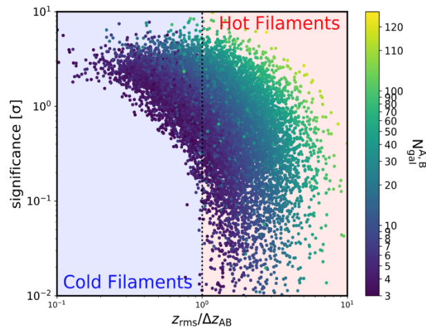
Simulation: TNG300-1
